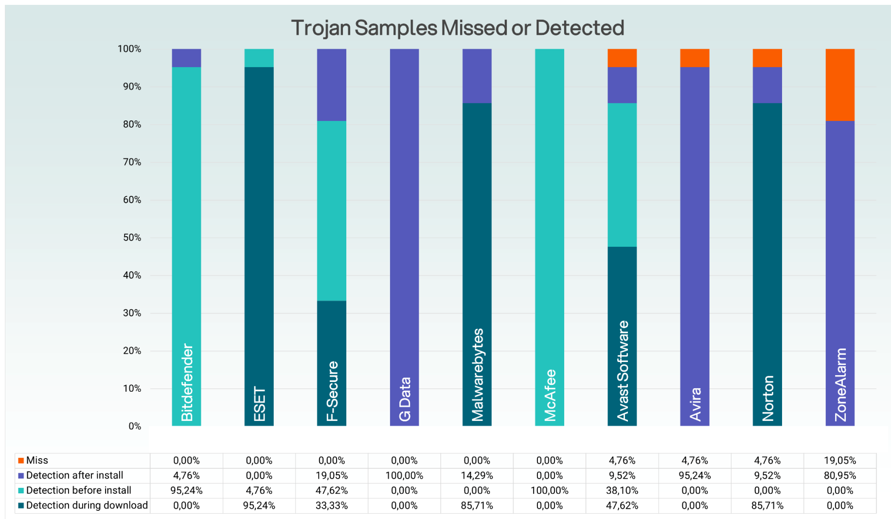
Figure 5. Summary, Trojan Samples
