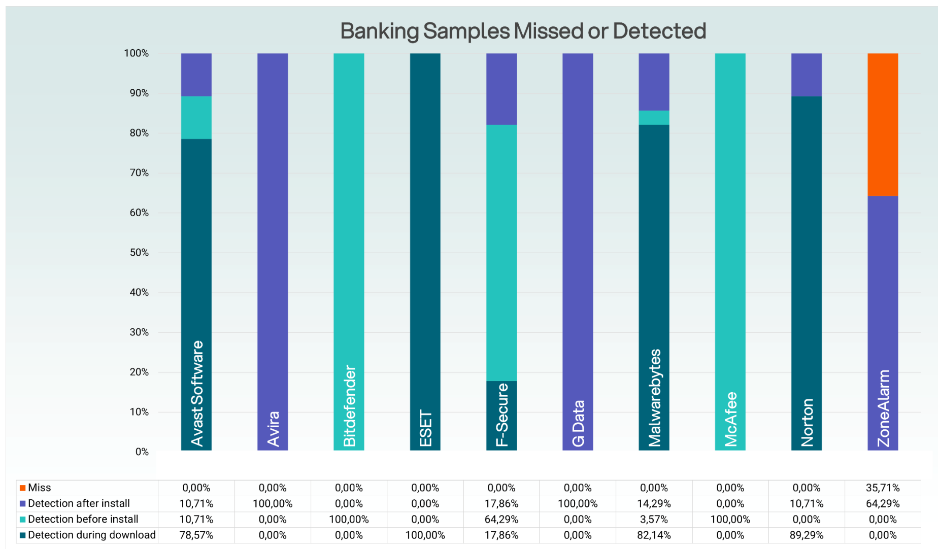
Figure 6. Summary, Banking Samples
