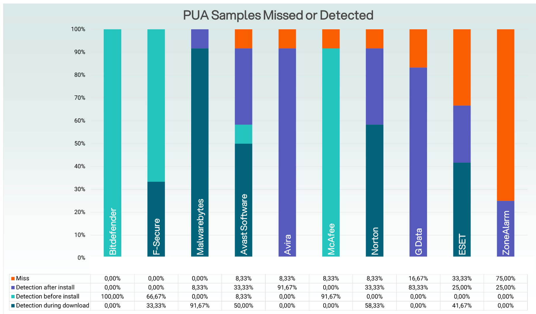
Figure 4. Summary, PUA Samples
