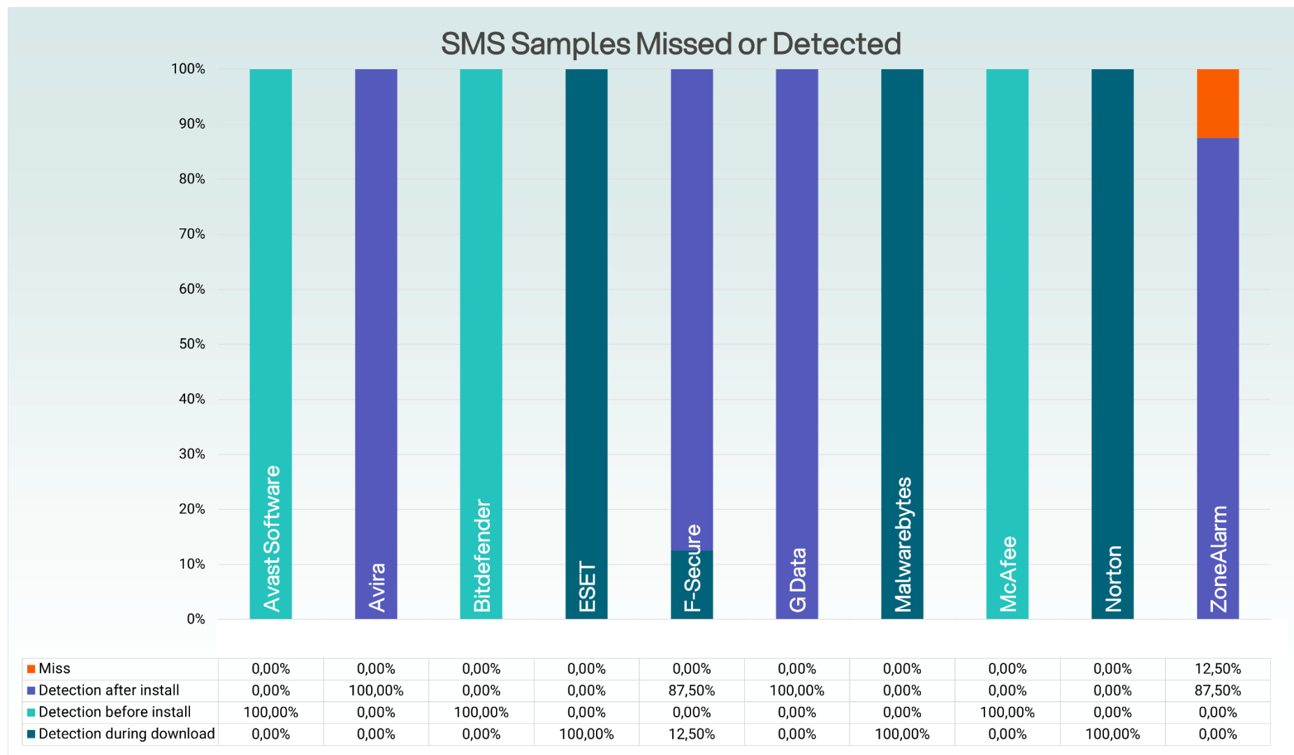
Figure 7. Summary, SMS samples
