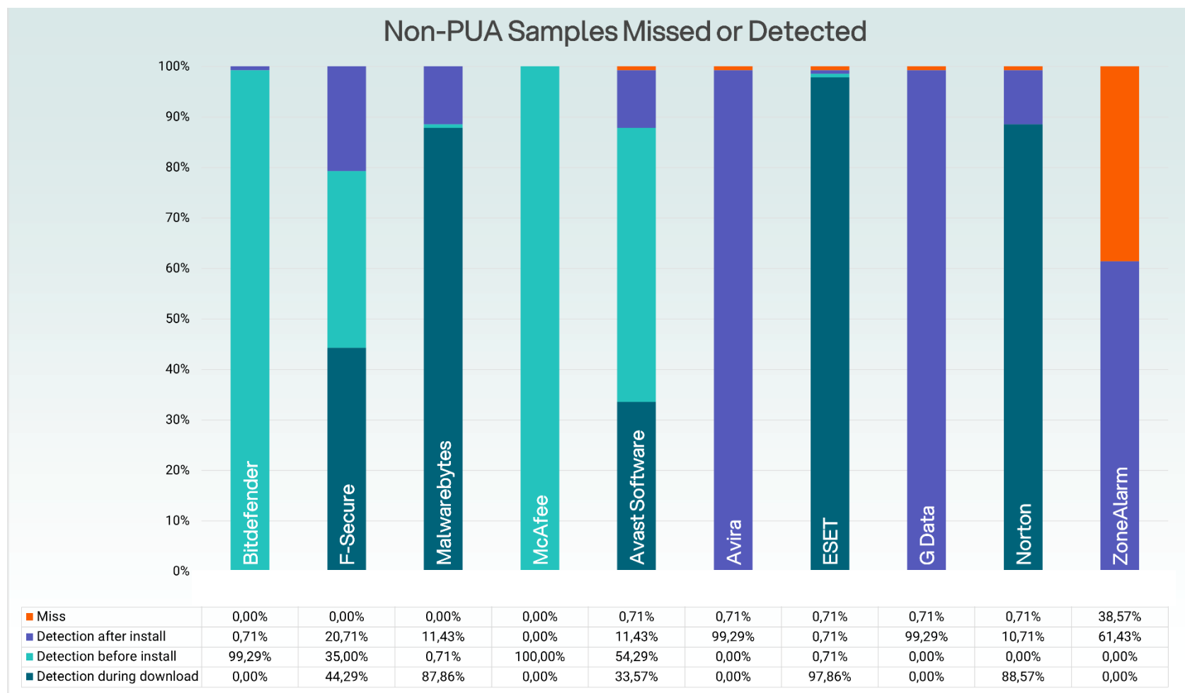
Figure 3. Summary, Non-PUA samples
