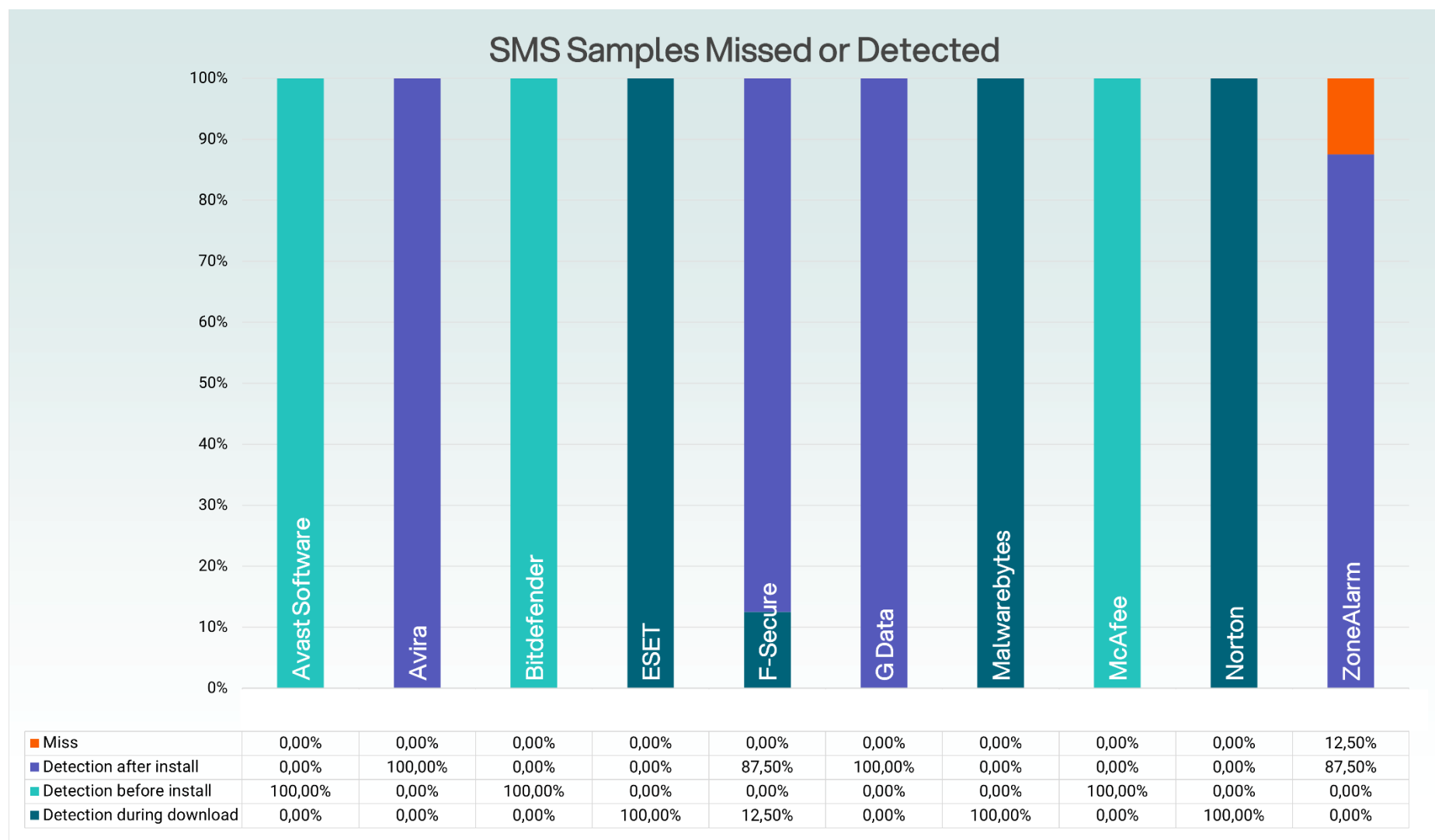
Figure 9. Summary, simulator samples
